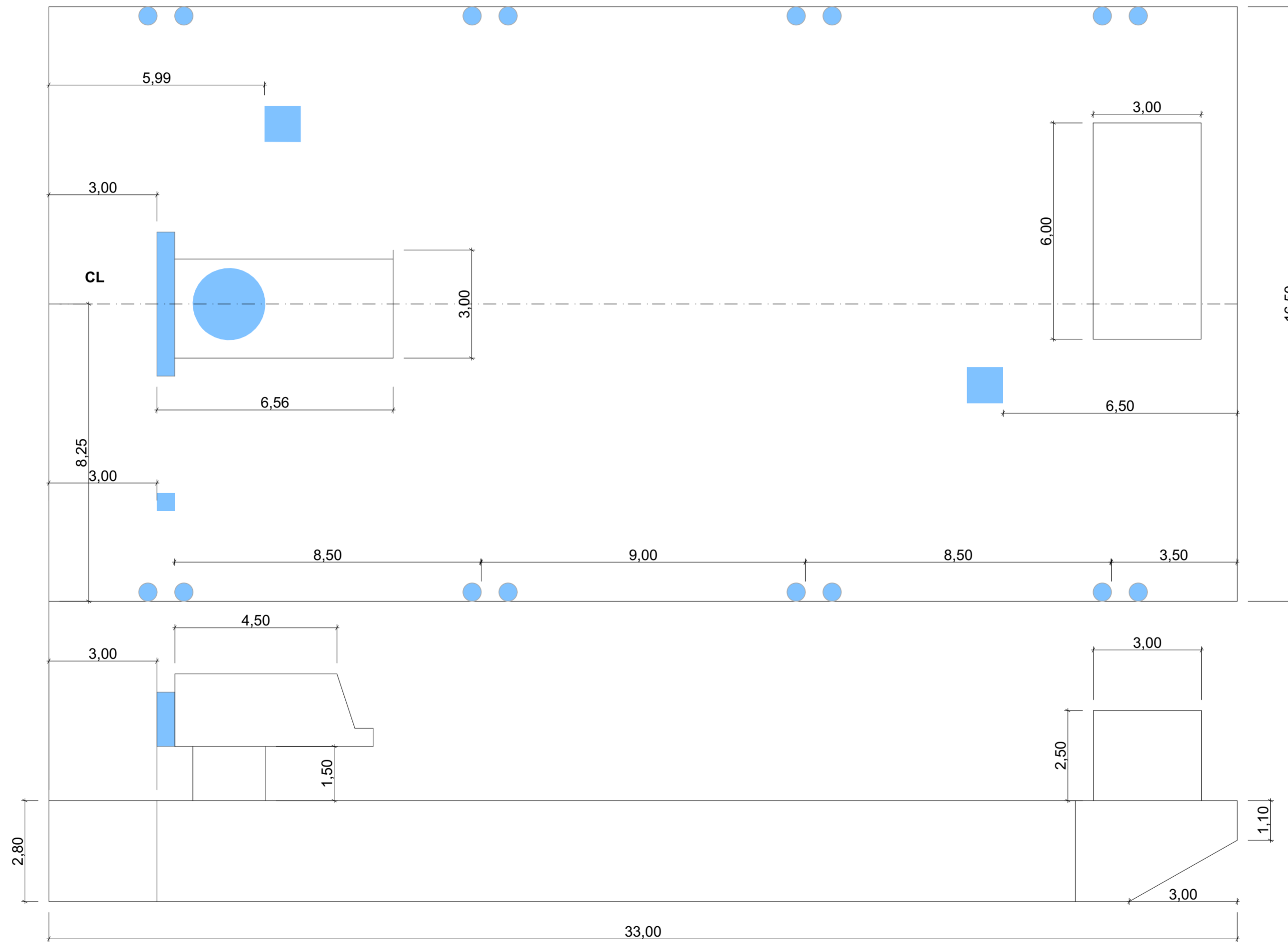
GENERAL ARRANGEMENT FLOATING CRANE HRAKLHS NB 01 L.O.A 33m BREADTH 16.5m DEPTH 2.8m SCALE 1:100
